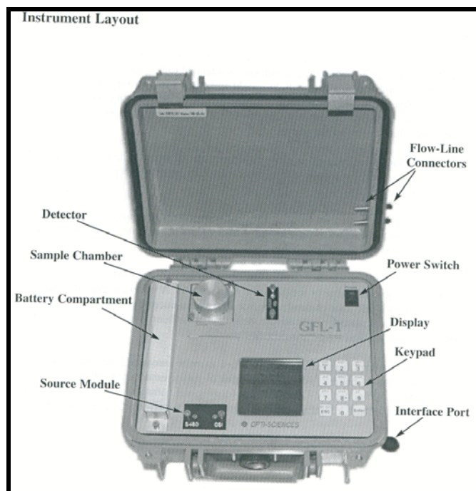
Figure F3.2: GFL-1 Portable Field Fluorometer
